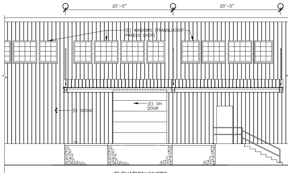
ELEVATION WH3B2
