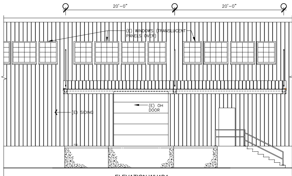
ELEVATION WH1B4
