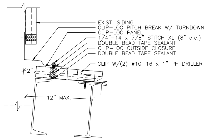
3 WALL TO ROOF FLASHING -- 1-1/2" = 1'-0"
