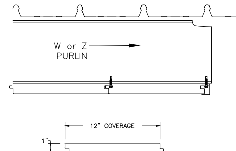
6 SOFFIT PANEL -- 1"=1'-0"
