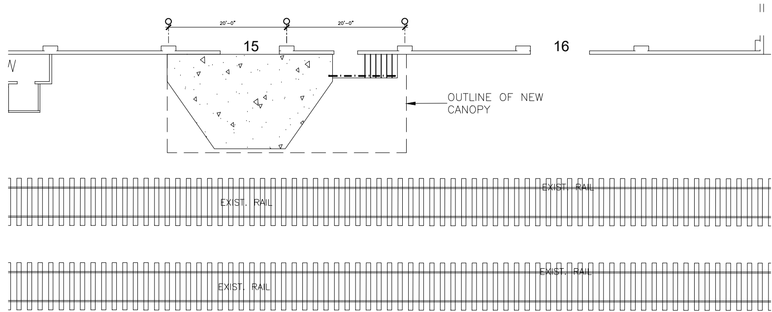
1 PLAN VIEW WH1B4 1/16"=1'-0"
