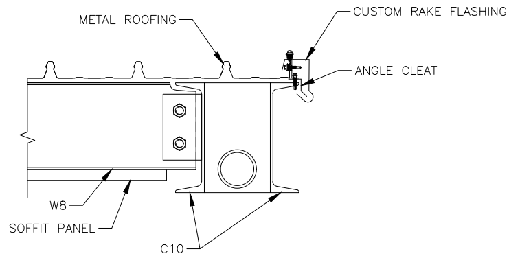
1 RAKE OFF MODULE W SECTION -- 1"=1'-0"
